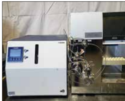
Gilson CPC Isolate and PLC2500 Flash Chromatography System
