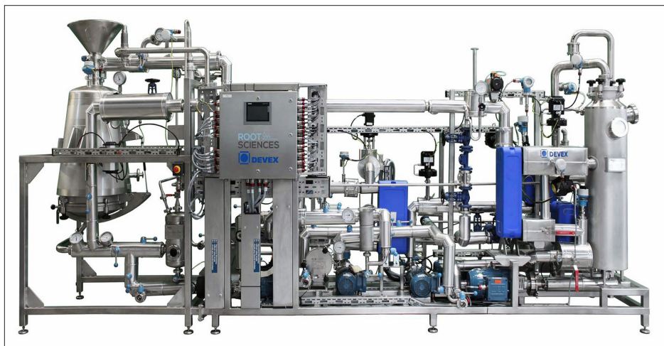
Root Sciences CryoExs 400 Cro Ethanol Extraction System
